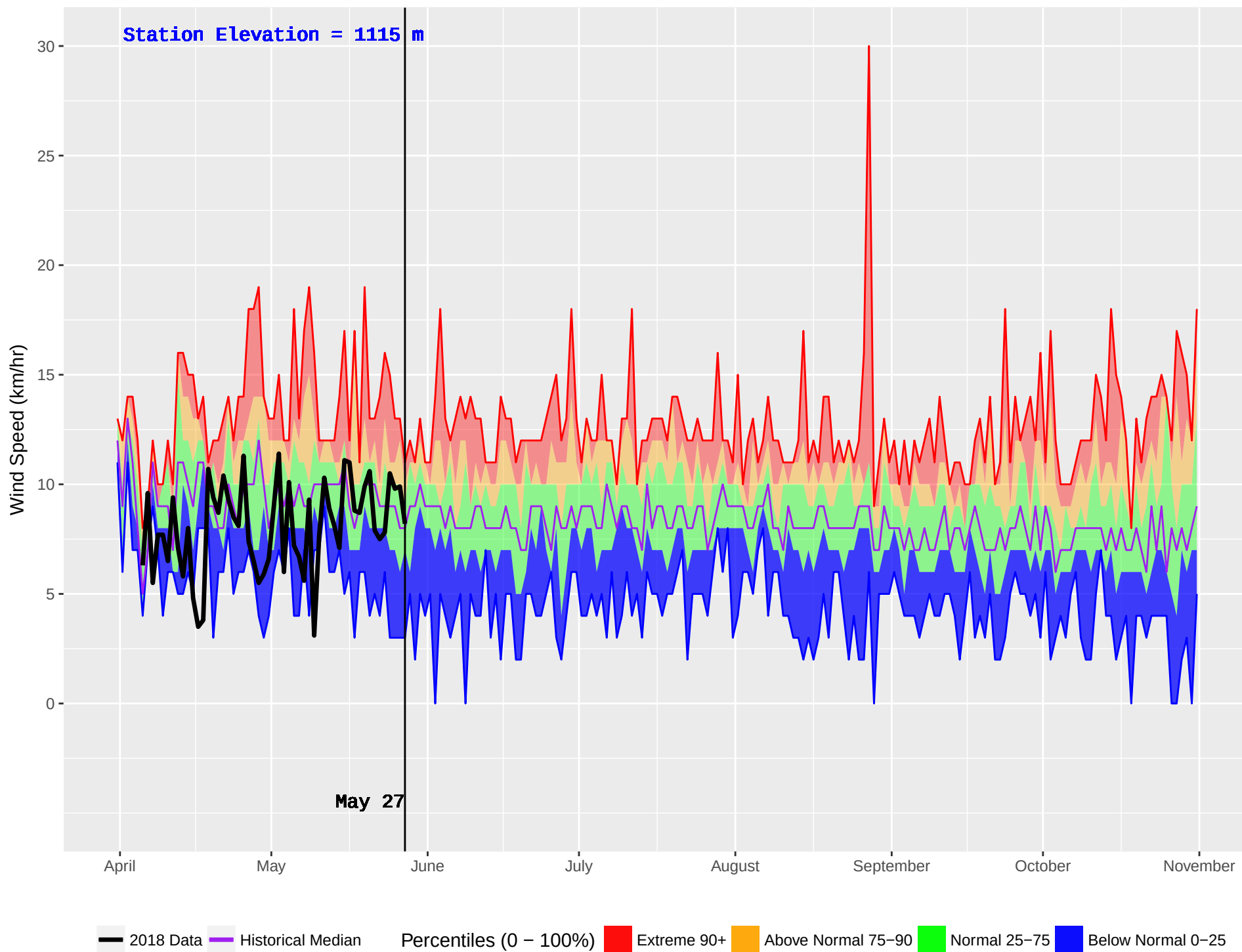
SICAMOUS (882) : Historical (2004–2016) and Current (2018) Noon Wind Speed
