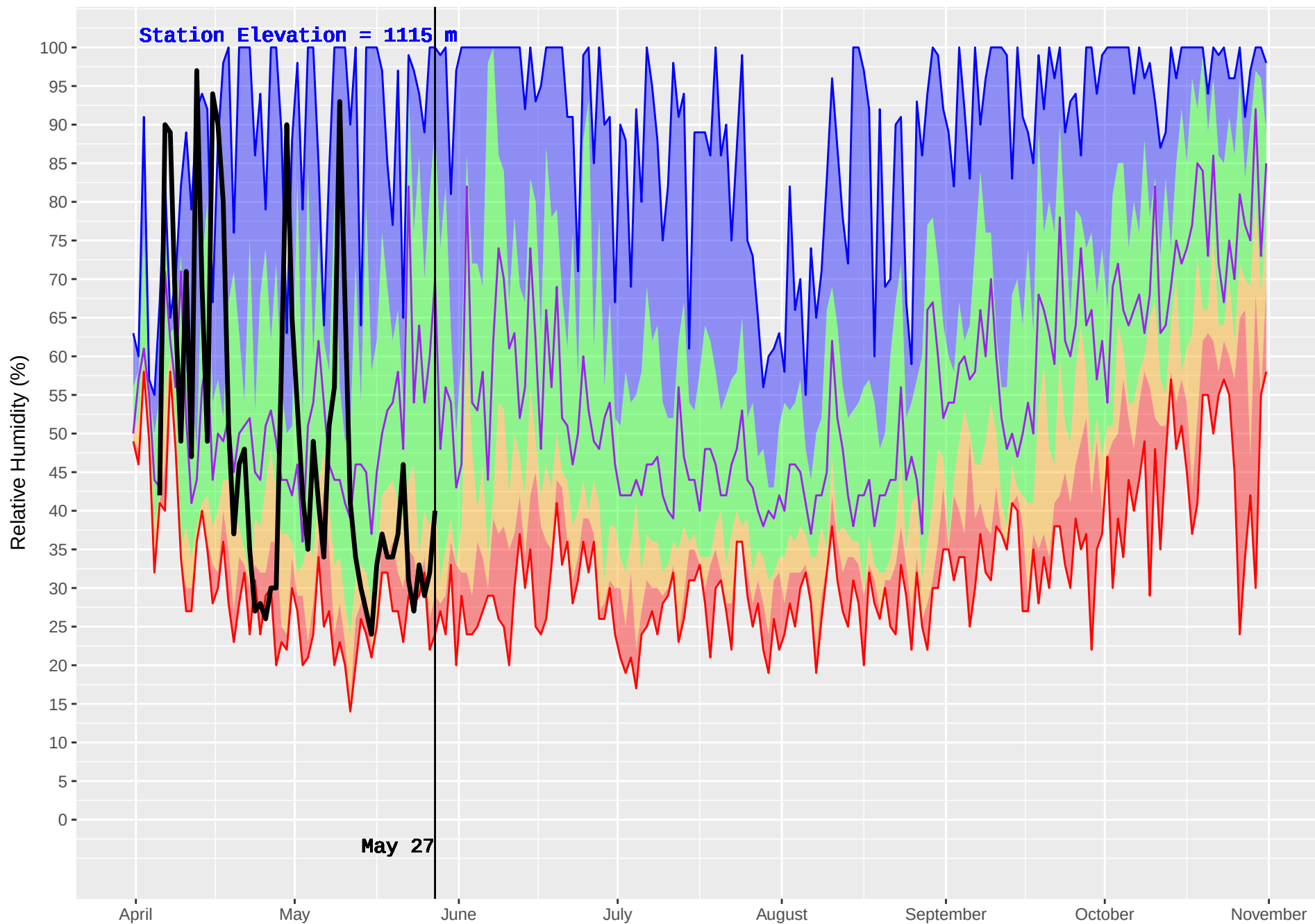
SICAMOUS (882) : Historical (2004–2016) and Current (2018) Noon Relative Humidity
