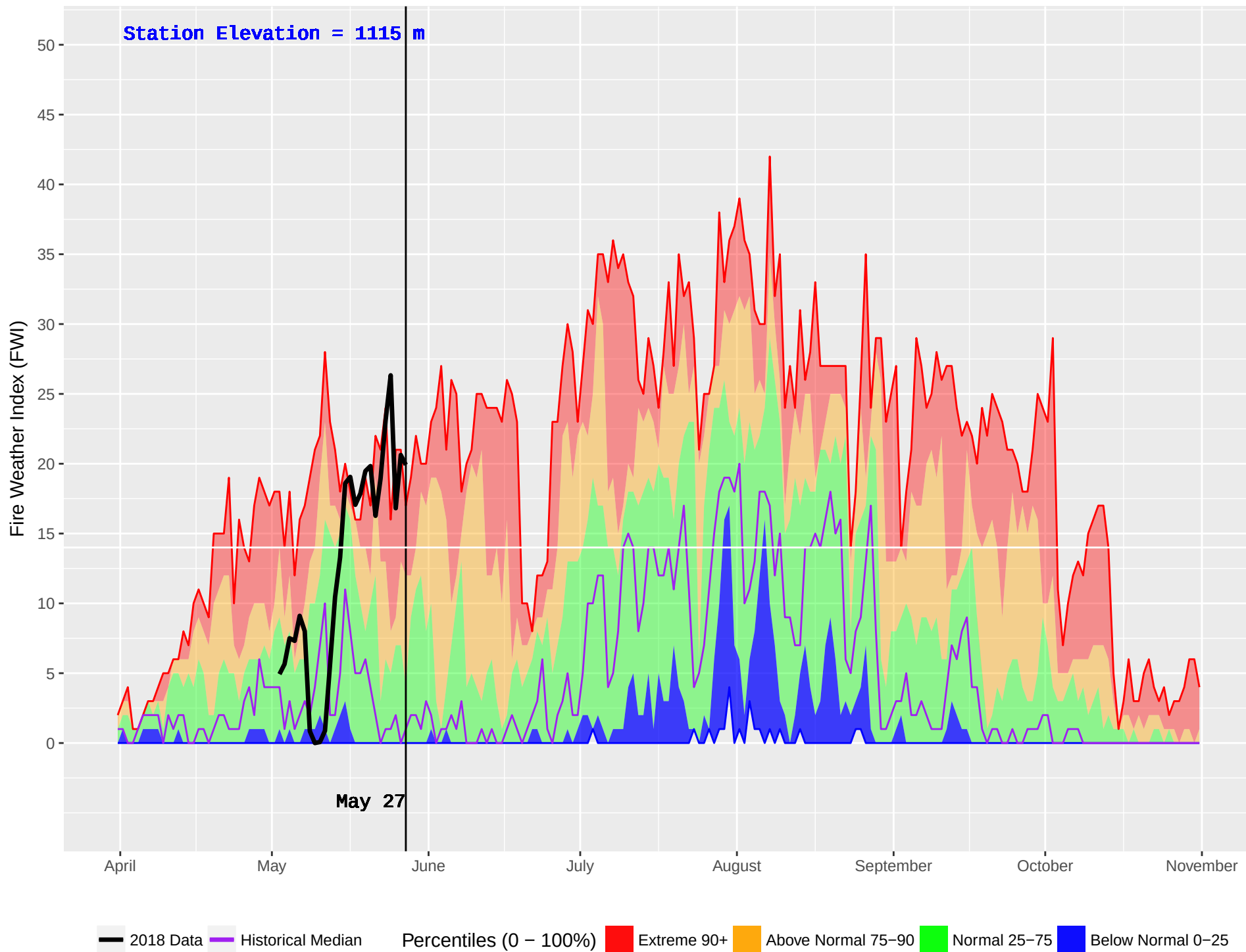
SICAMOUS (882) : Historical (2004–2016) and Current (2018) Noon Fire Weather Index (FWI)
