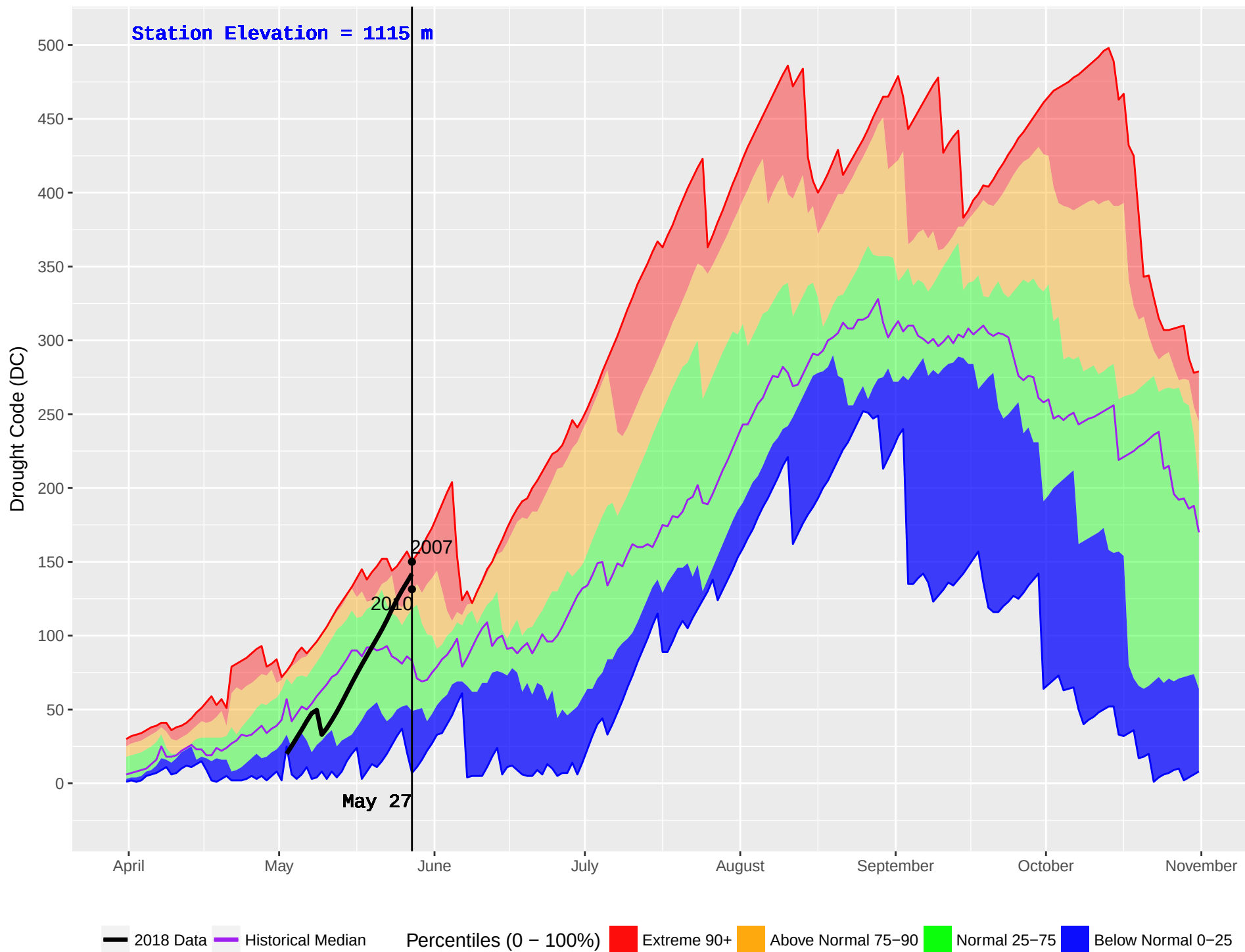
SICAMOUS (882) : Historical (2004–2016) and Current (2018) Noon Drought Code (DC)
