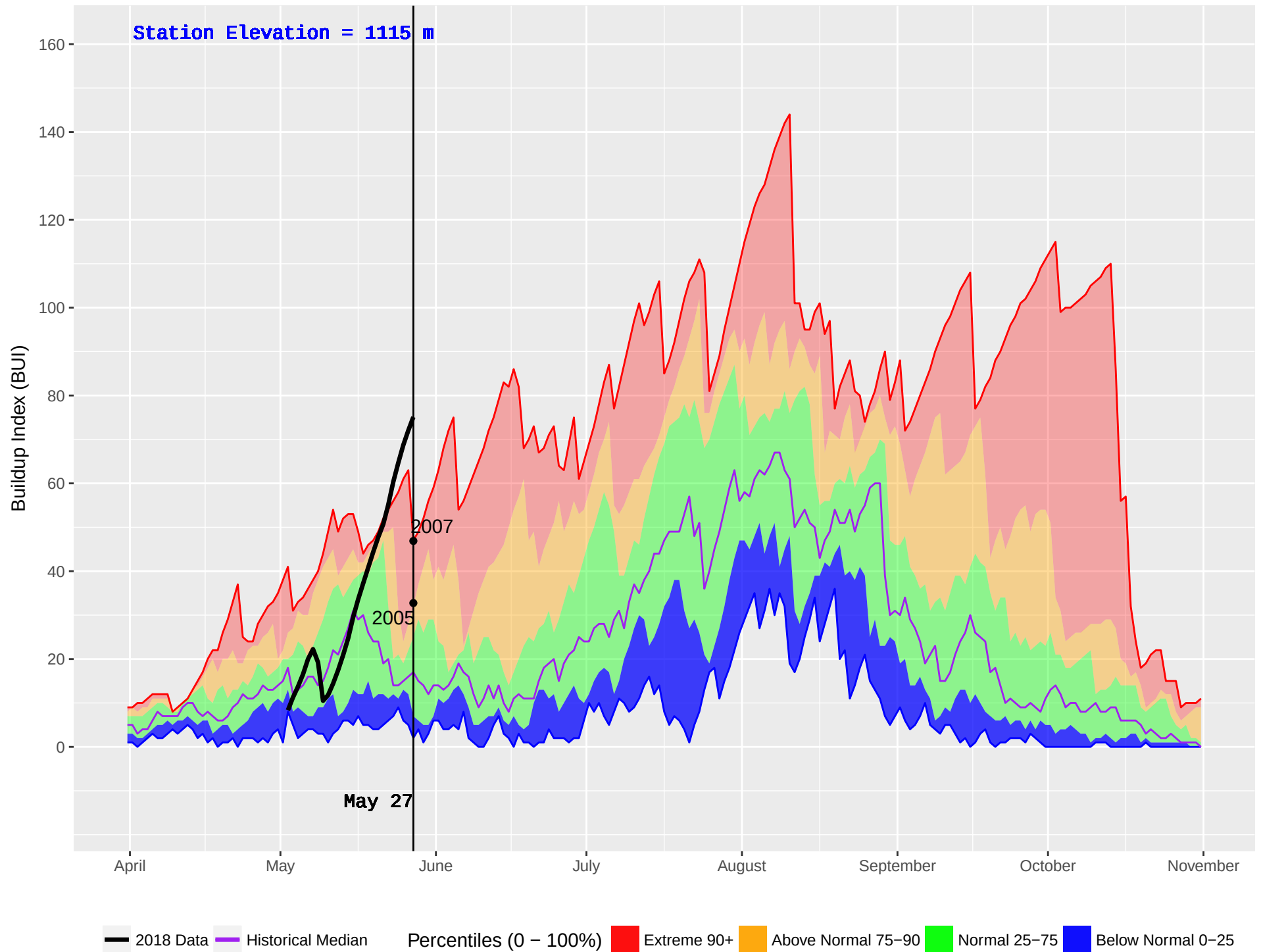
SICAMOUS (882) : Historical (2004–2016) and Current (2018) Noon Buildup Index (BUI)
