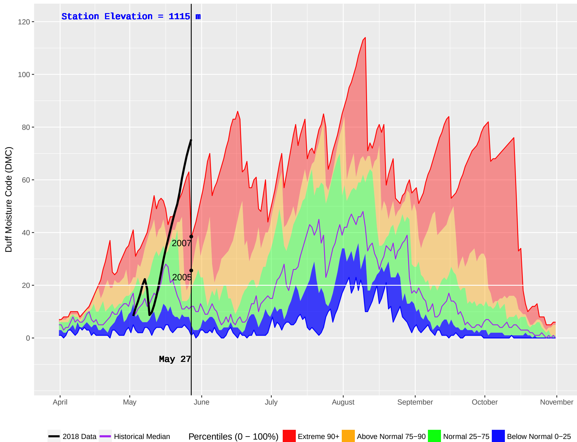
SICAMOUS (882) : Historical (2004–2016) and Current (2018) Noon Duff Moisture Code (DMC)
