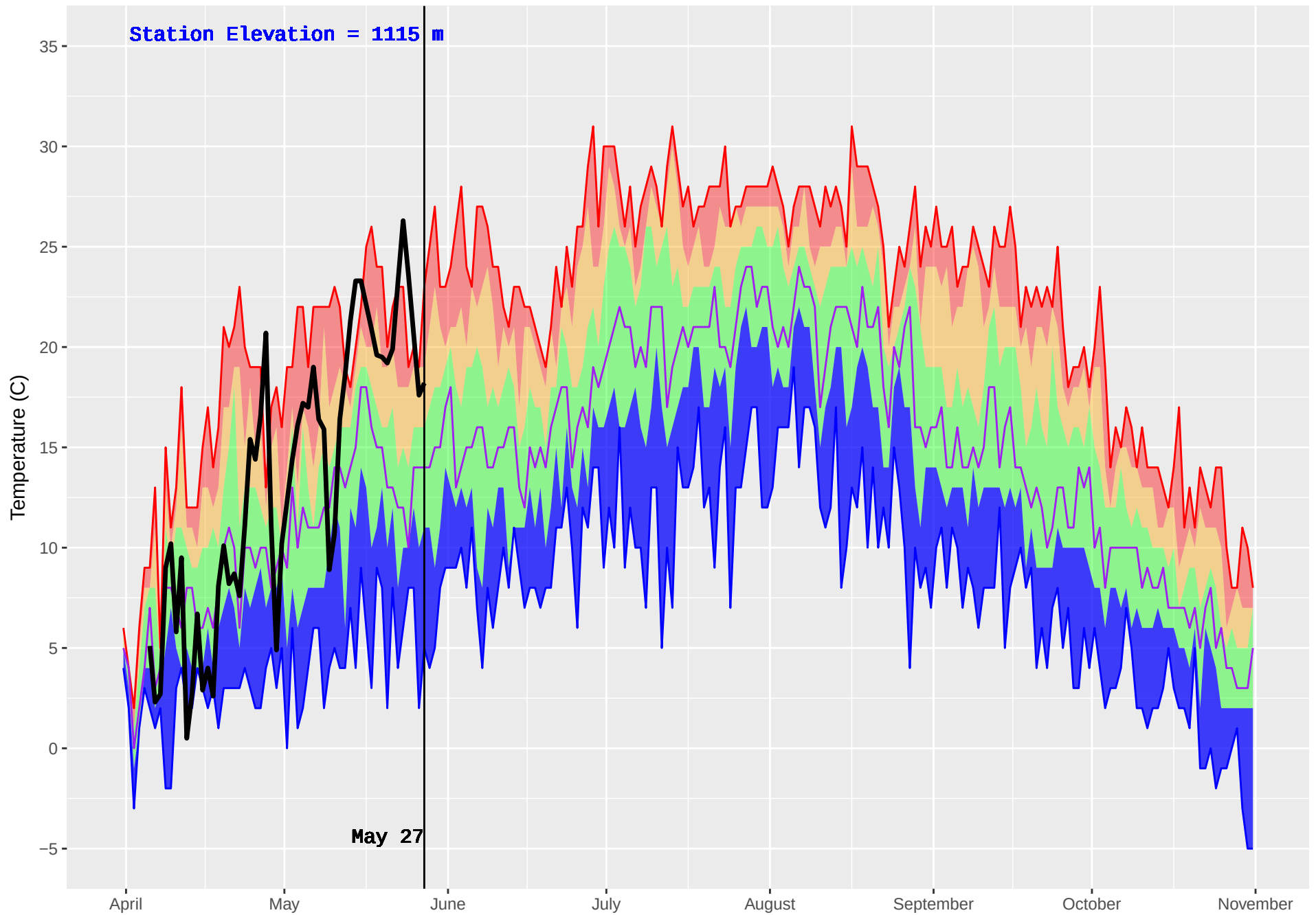
SICAMOUS (882) : Historical (2004–2016) and Current (2018) Noon Temperature
