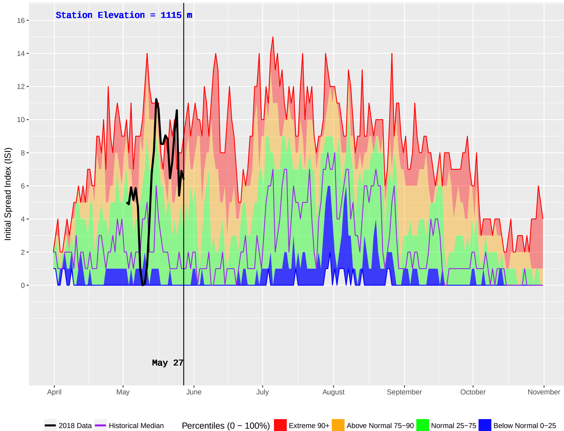
SICAMOUS (882) : Historical (2004–2016) and Current (2018) Noon Initial Spread Index (ISI)
